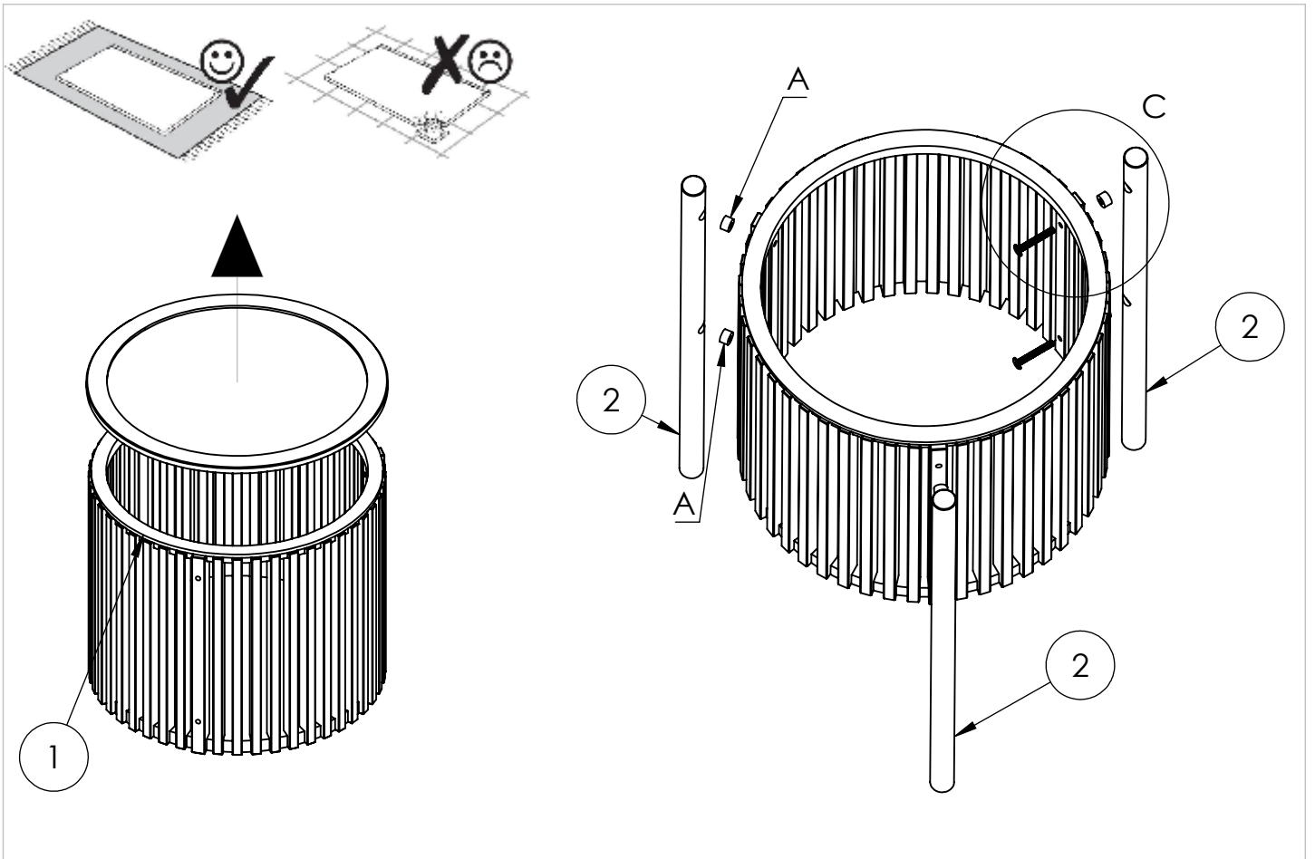
DETAIL C
