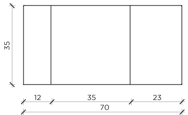
FRONTE | FRONT
