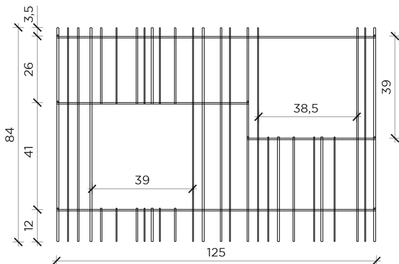
FRONTE | FRONT
